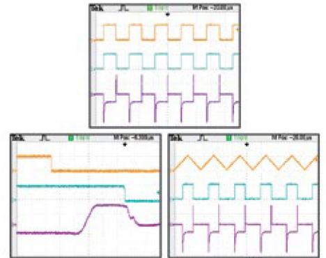
Oscillograms Testing the GDU with GTO and Freewheeling Diode
